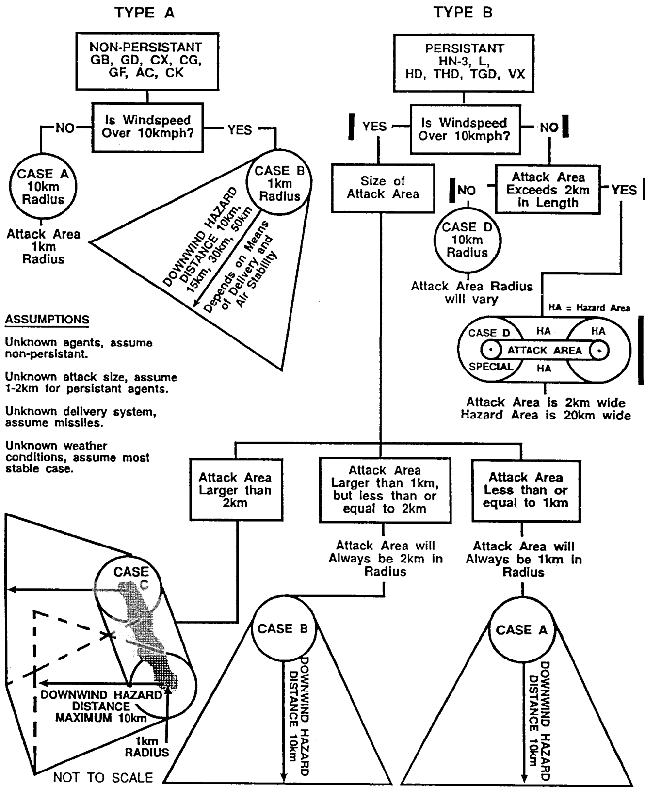
Flow Chart
